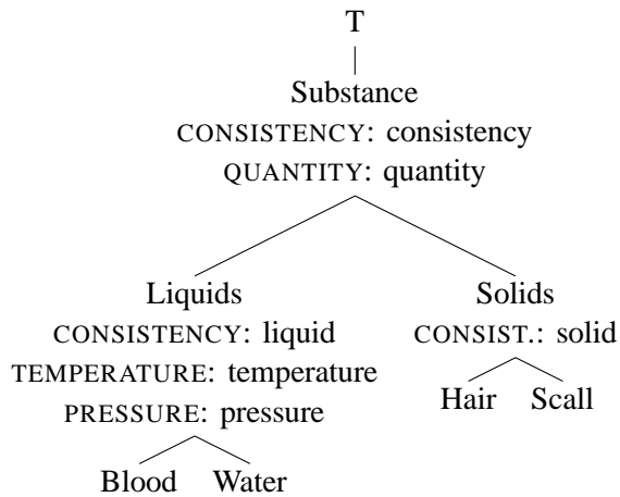
Figure 6: Partial type signature.
